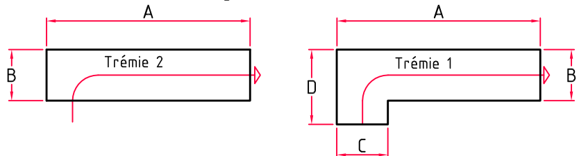
Configuration Trémie
