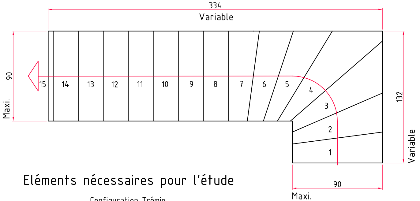
Configuration Trémie
