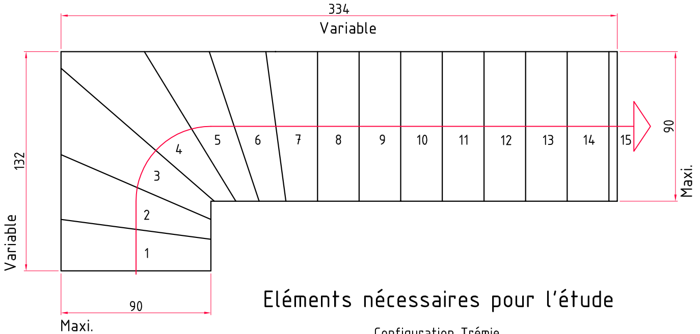
Configuration Trémie
