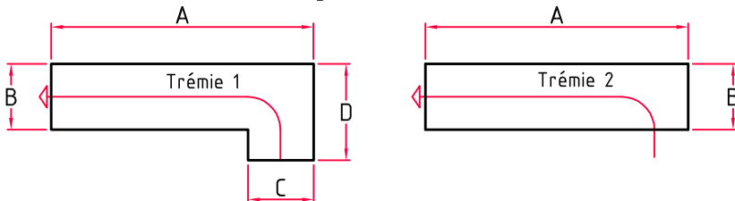
Configuration Trémie
